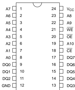
DS2016 24-PIN DIP (600 MIL) DS2016S 24-PIN SOIC (330 MIL)
